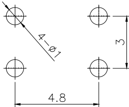
PCB.WELDING DRAWING
