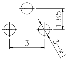
PCB.WELDING DRAWING
