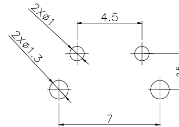
PCB.WELDING DRAWING
