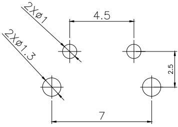
PCB.WELDING DRAWING
