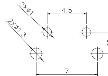
PCB.WELDING DRAWING
