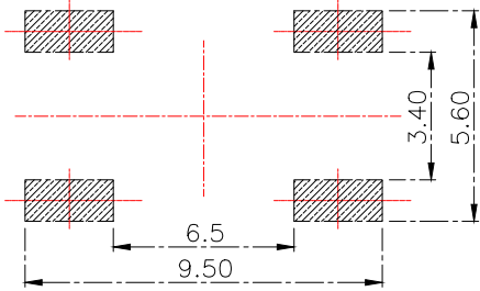
PCB.WELDING DRAWING
