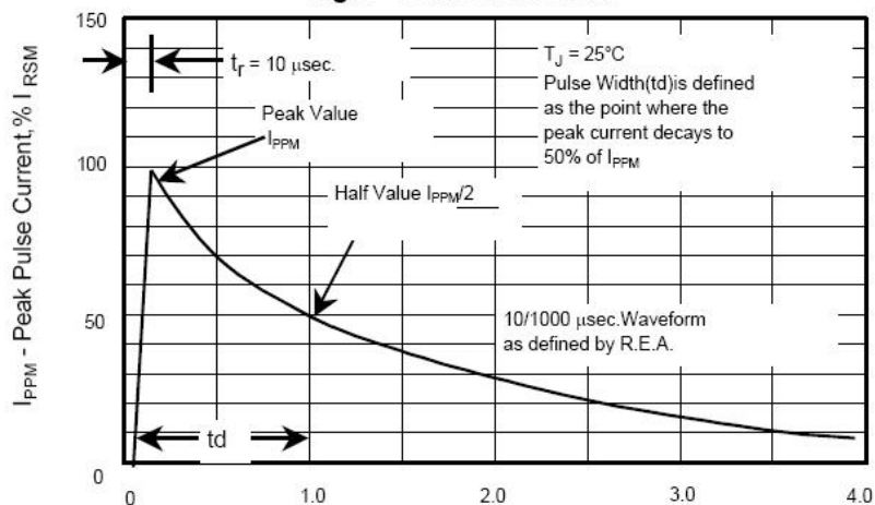
Fig.3 - Pulse Waveform
