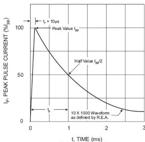
Fig. 4 Pulse Waveform
