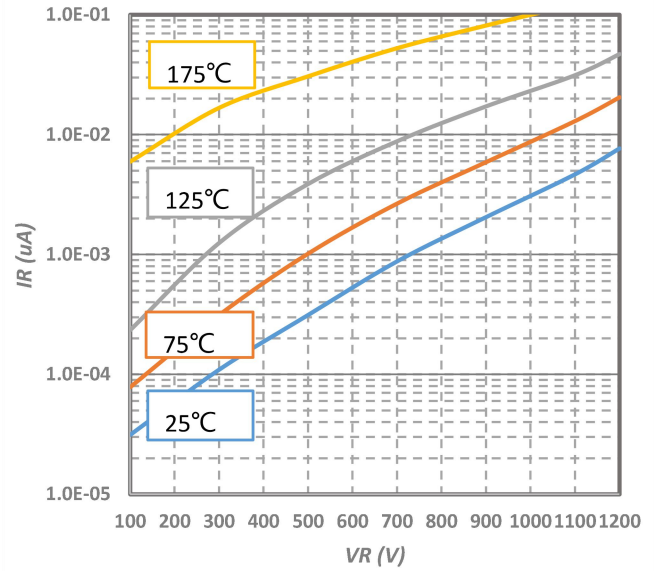
Fig.2-Typical Reverse Characteristics
