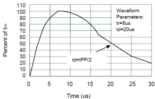
Pulse Waveform
