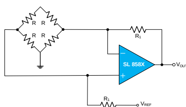
Figure 5. Bridge Amplifier
