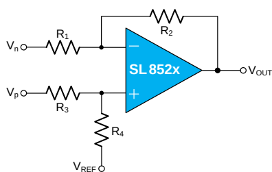
Figure 5. Differential Amplifier
