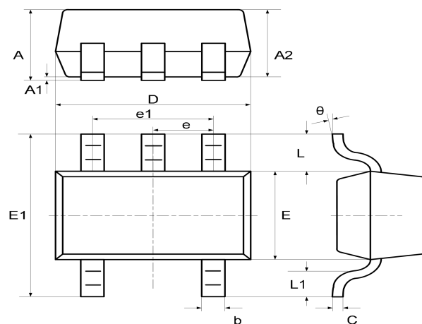
SC70-5
