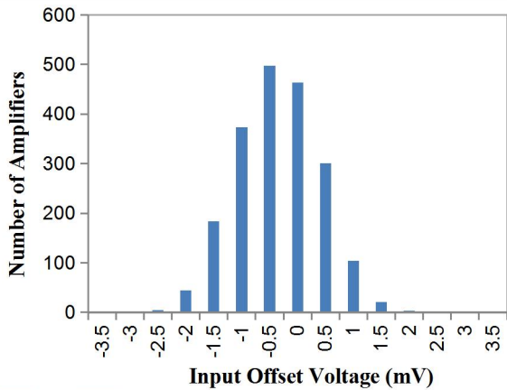
Figure 4 Input Offset Voltage Production Distribution
