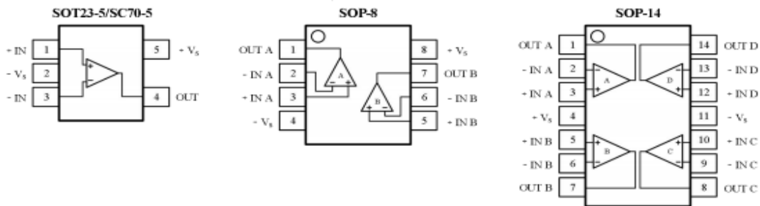
Figure 1 Pin Configurations
