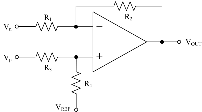
Figure 14 Differential Amplifier
