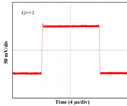
Figure 9 Small-Signal Step Response at 5V
