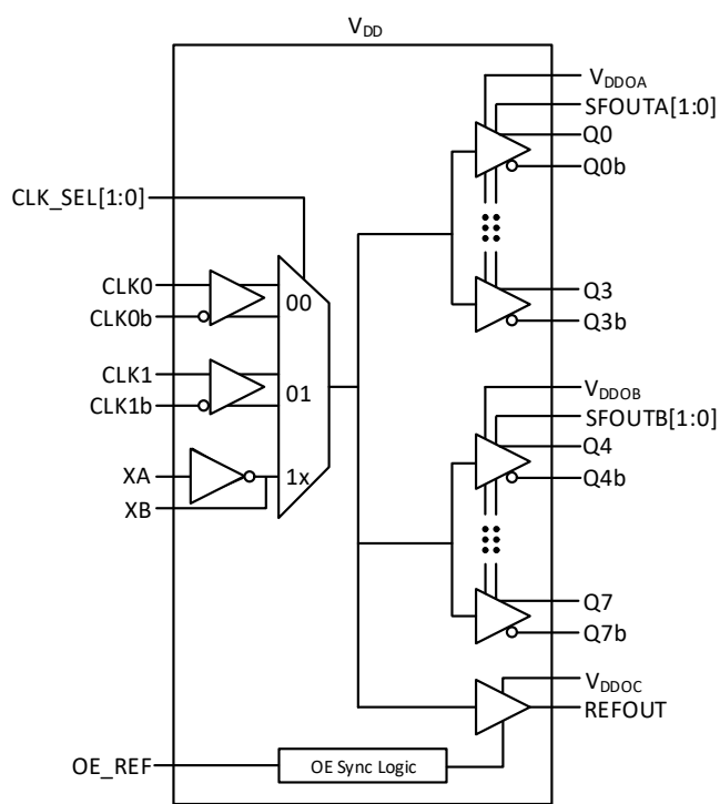
Figure 6. SKY53580 Block Diagram
