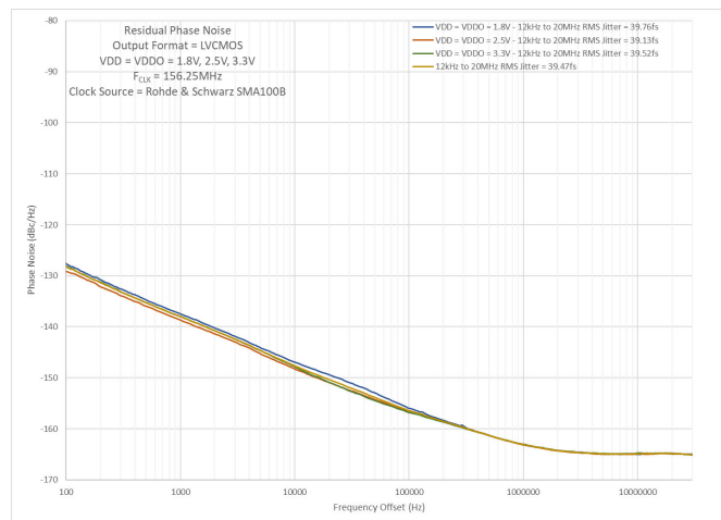
Figure 48. Residual Phase Noise Differential Input (REFOUT: 156.25 MHz)
