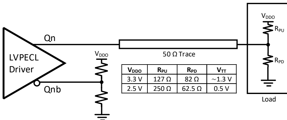
Figure 27. Single-Ended LVPECL Clock Output Termination, DC Coupling (Thevenin Equivalent)
