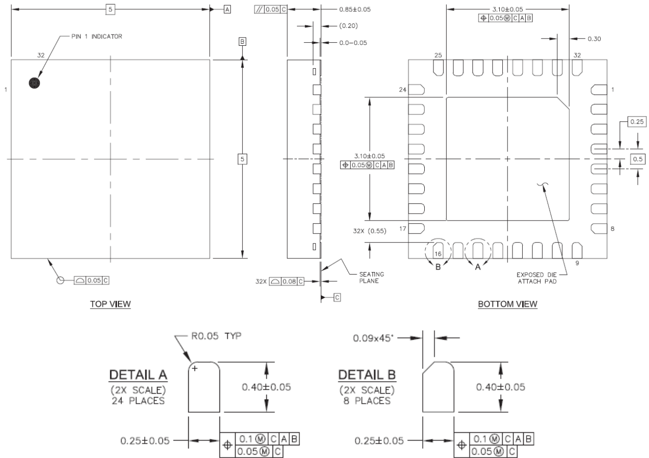
Figure 64. 5x5 mm 32-QFN Package Dimensions
