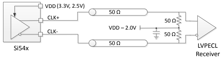
DC-Coupled LVPECL - 50 Ω w/VTT Bias
