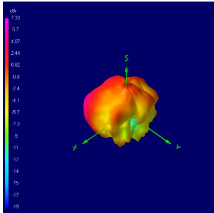
3625 MHz
