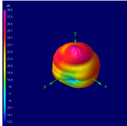
1176.45 MHz
