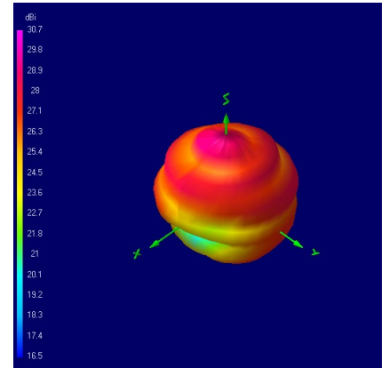
1561.098 MHz
