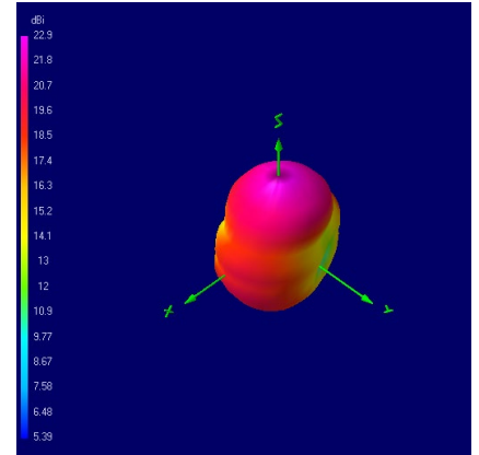
1207.14 MHz
