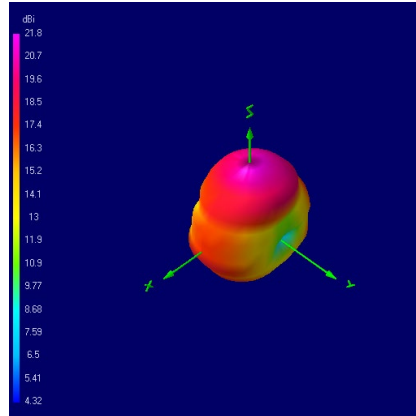
1202.025 MHz
