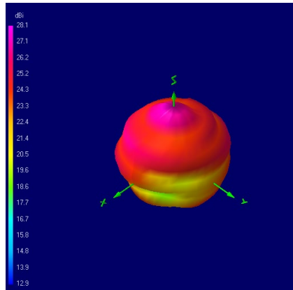
1575.42 MHz
