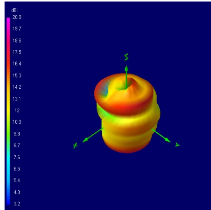
1246 MHz
