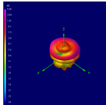
5482 MHz
