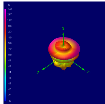
5570 MHz
