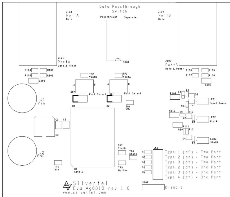
Figure 1: EvalAg6810 Board Layout
