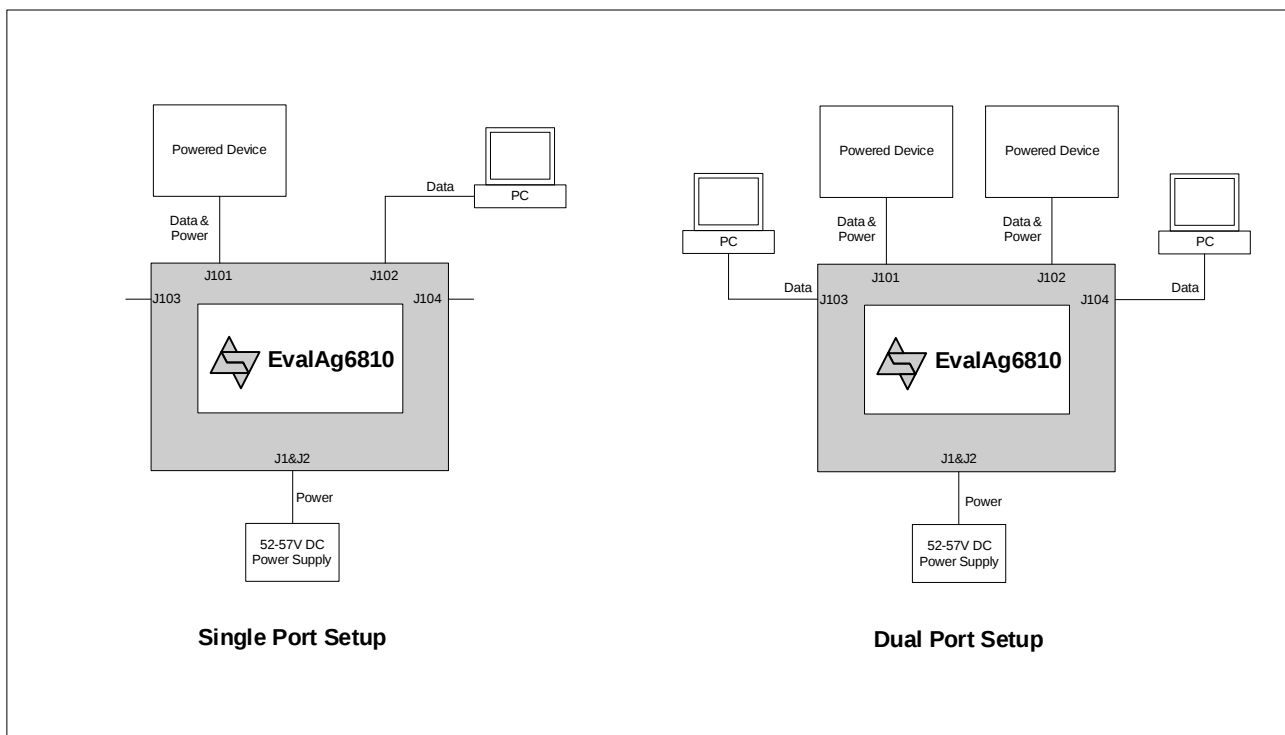
Figure 2 Basic Test Setup
