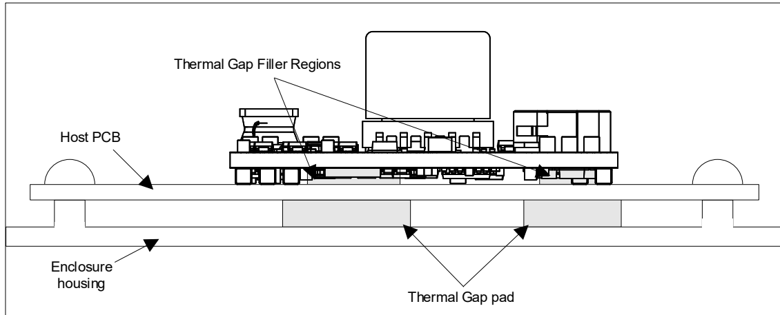
Figure 9: Additional Heatsinking
