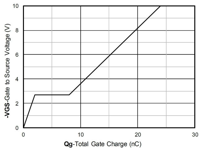
Gate Charge
