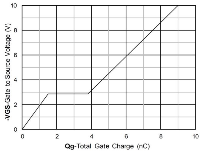
Gate Charge
