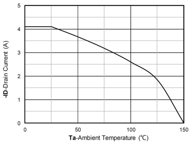
Current dissipation
