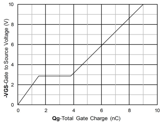
Gate Charge
