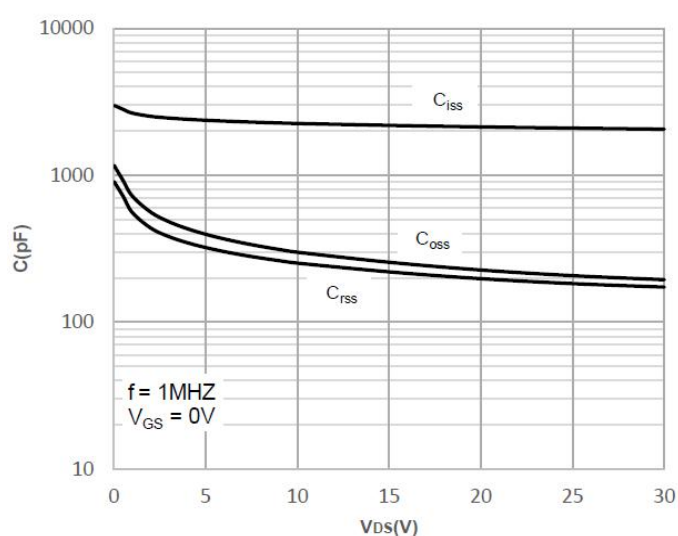
Capacitance Characteristics
