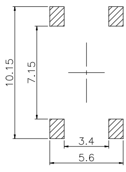
PCB. 焊接图 PCB. WELDING DRAWING
