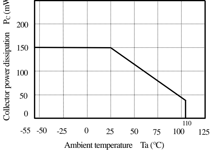
(Fig. 3) Collector power dissipation vs. ambient temperature
