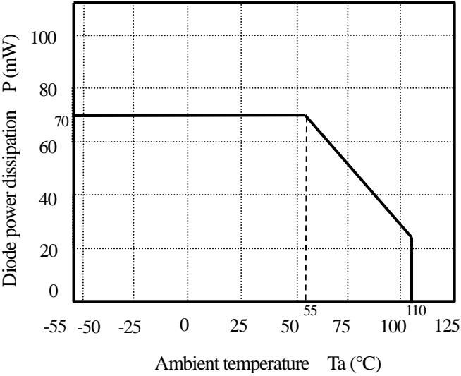
(Fig. 4) Total power dissipation vs. ambient temperature
