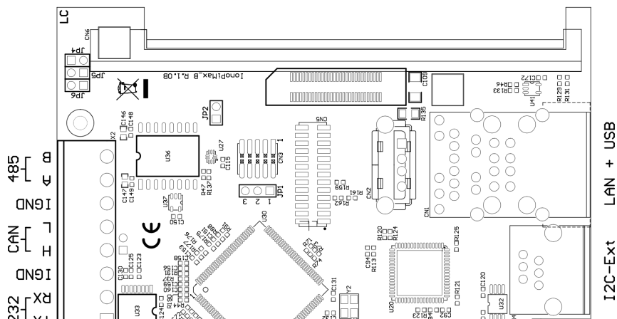
SWD JUMPERS
