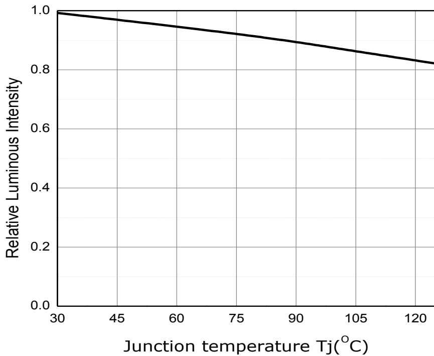
Fig 6. Junction Temperature vs. Relative Luminous Intensity, I_F=100\text{mA}
