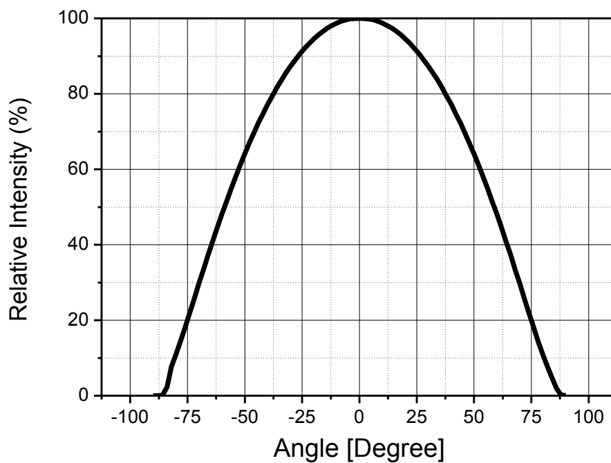
Fig 2. Radiant Pattern, T_j = 25^{\circ}\text{C} , I_F = 100\text{mA}
