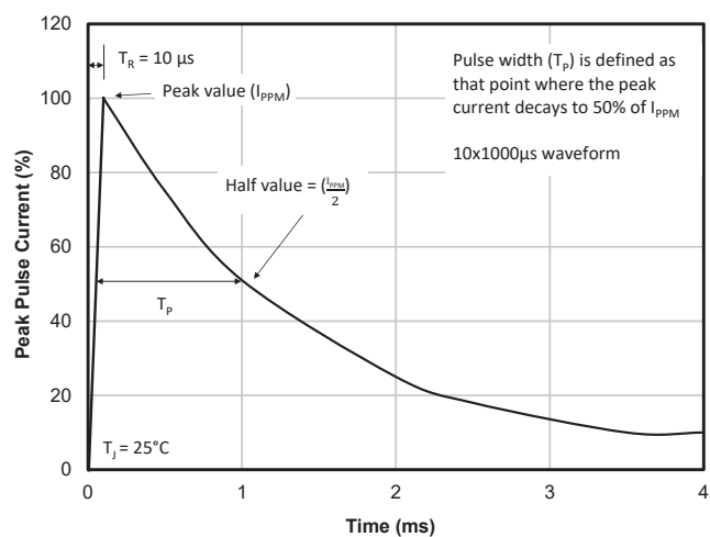
Pulse Waveform
