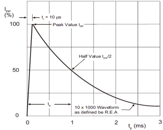
Figure 2. Pulse waveform
