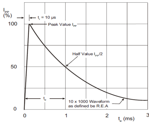
Figure2. Pulse waveform
