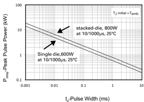
Figure 3. Peak pulse power rating curve
