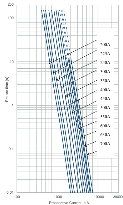
AL054, AL055, AL056 3853-R Bolt-on B, C and D, 200-700 A, 500 VDC
