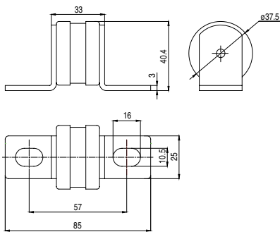
AL013 3734 Bolt-on A
