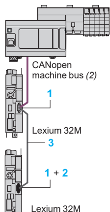
Lexium 32M Example of connecting Lexium 32M with VW3A3628 card
