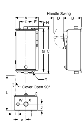
Figure 16.4: NEMA 1 Enclosure, Size 0–2 Figure 16.5: NEMA 1 Enclosure, Size 3–6 Figure 16.6: NEMA 12 Enclosure Figure 16.7: NEMA 4X Stainless Steel Enclosure
