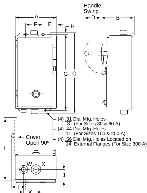
Figure 16.26: NEMA 4, 4X Enclosure
