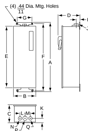
Figure 16.23: Night-Master Style
