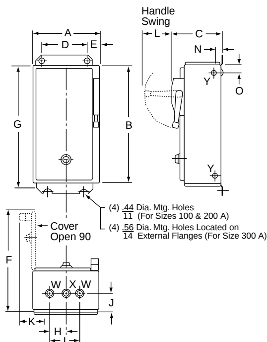
Figure 16.25: NEMA 1 Enclosure
