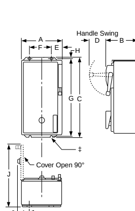
Figure 16.4: NEMA 1 Enclosure, Size 0–2 Figure 16.5: NEMA 1 Enclosure, Size 3–6 Figure 16.6: NEMA 12 Enclosure Figure 16.7: NEMA 4X Stainless Steel Enclosure
