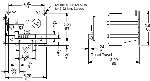
NEMA Size 00B, 00C, 0, and 1 Devices
