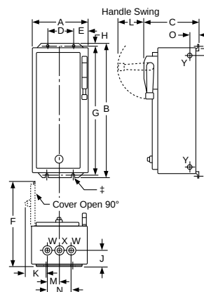
Figure 16.4: NEMA 1 Enclosure, Size 0–2 Figure 16.5: NEMA 1 Enclosure, Size 3–6 Figure 16.6: NEMA 12 Enclosure Figure 16.7: NEMA 4X Stainless Steel Enclosure
