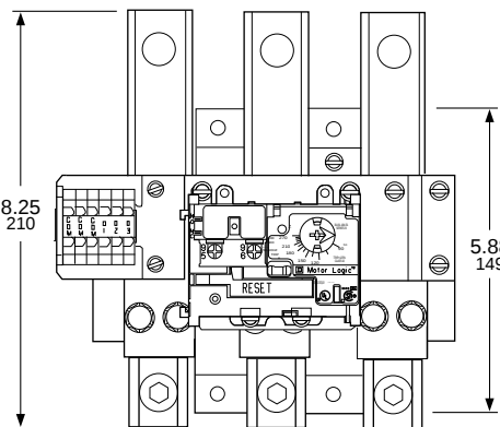
NEMA Size 5 Type S Device
