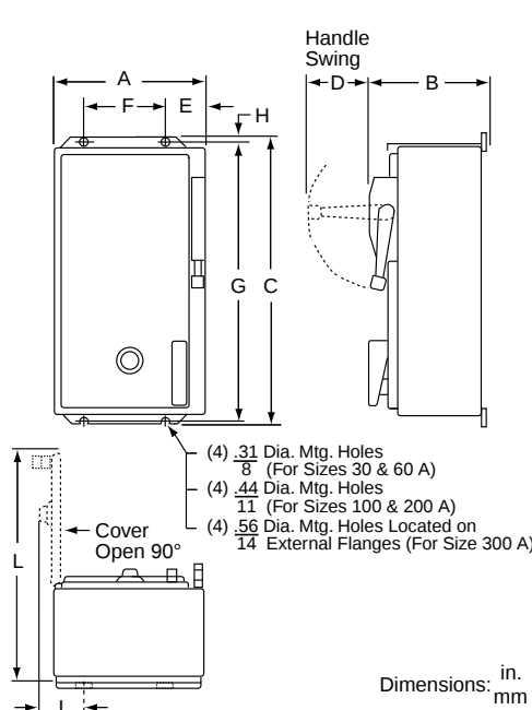
Figure 16.27: NEMA 12/3R Enclosure
