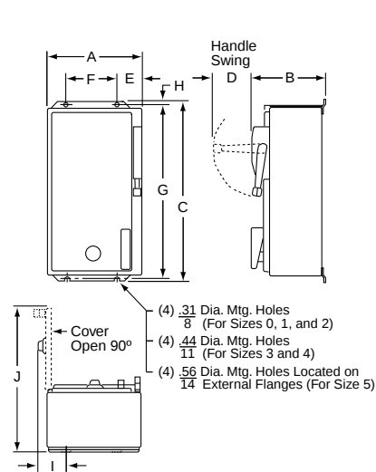
Figure 16.17: NEMA 12/3R Enclosure
