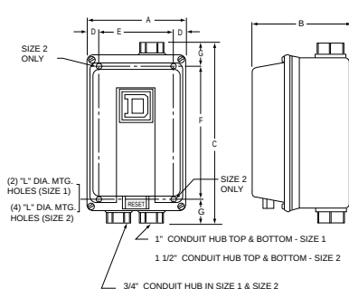
Figure 7: NEMA 4X—Watertight and Corrosion Resistant Glass Polyester Enclosures, Sizes 0-2, without Form FF4T
