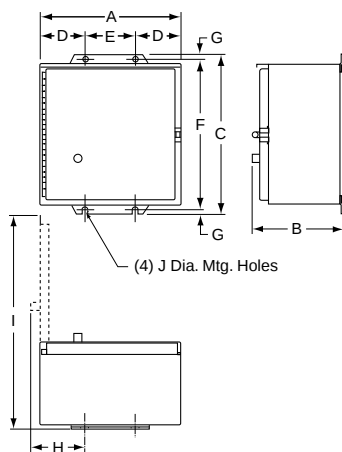
Figure 16.14: NEMA 12/3R
