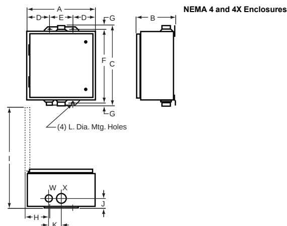
NEMA 4 and 4X Enclosures
