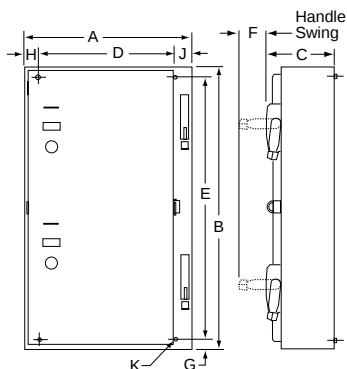
Figure 16.29: NEMA 1 Enclosure—Combination
