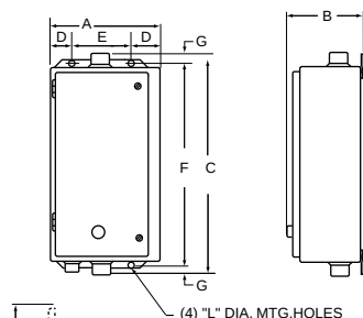
Figure 6: NEMA 4X—Stainless Steel Watertight Enclosure
