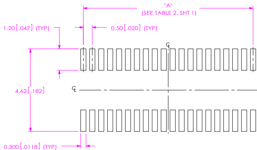
FIG 2 -20 POS SHOWN
