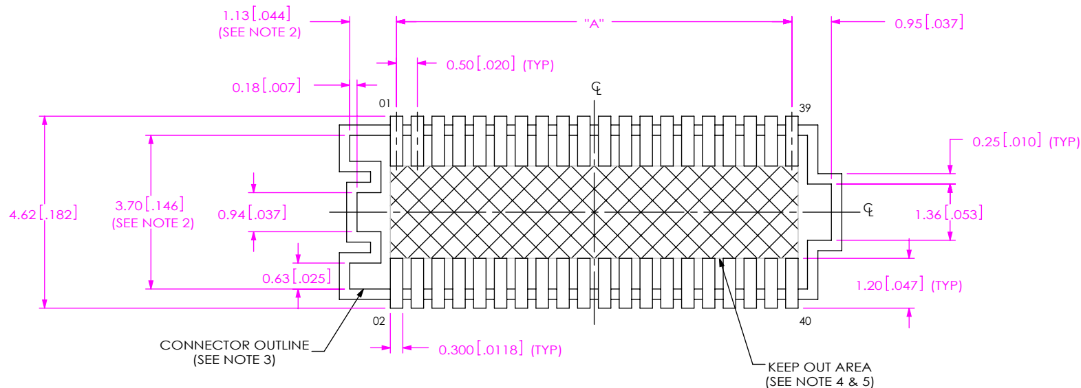
FIG 1 -20 POS SHOWN
