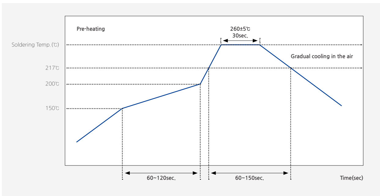
[Reflow Soldering Conditions]
