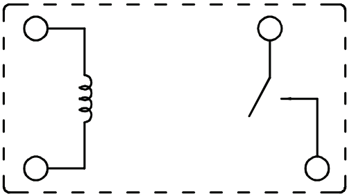
Wiring Diagram Bottom View
