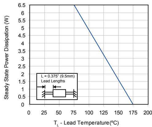
Figure 5 - Steady State Power Derating Curve
