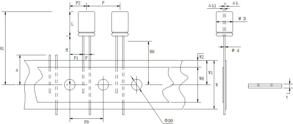
[ Fig. 4 (Diameter for Φ10 )
