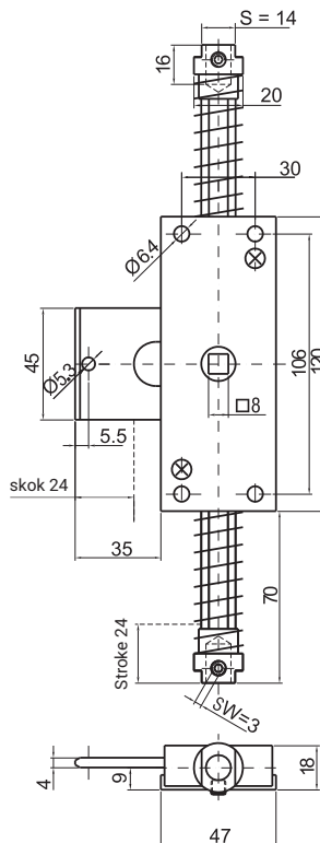
ZWM8 (with hole \varnothing 8 ) S = 14
