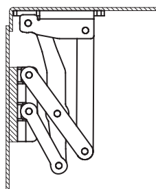
Closed position
