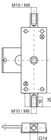
ZWM8 ZWM10 (with thread M8 ) (with thread M10 )
