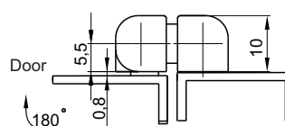
LEFT VERSION
