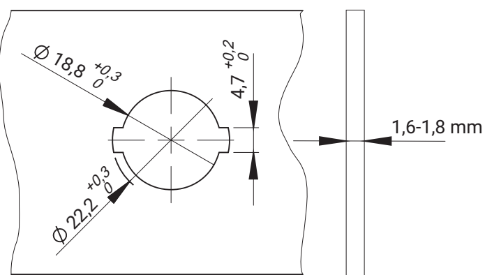
Cut out
