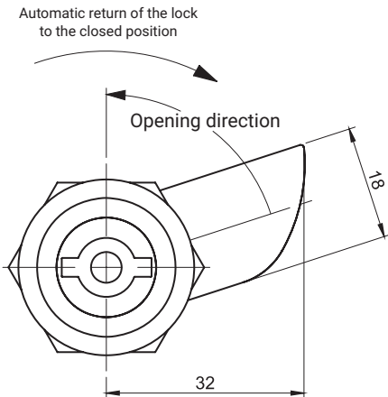
Lock in the left version, the right version is a mirror reflection
