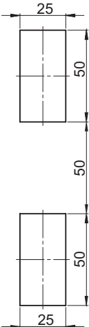
Mounting hole
