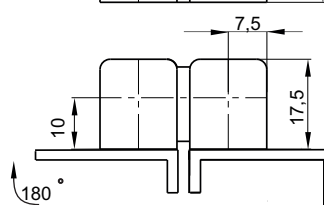
LEFT VERSION
