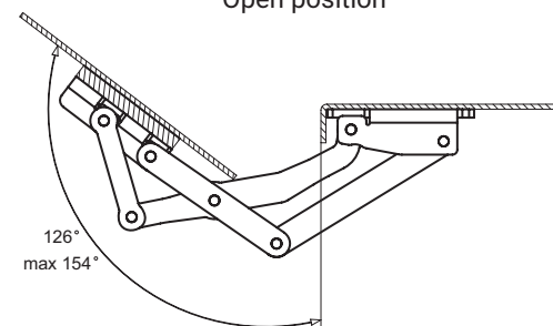
Open position
