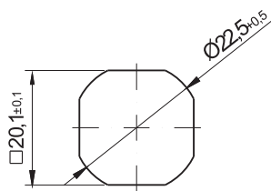
Cut out
