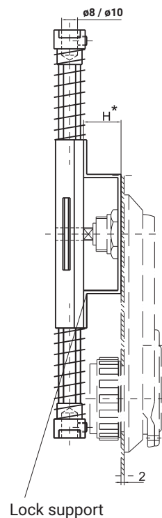
ZWM10 (with hole \varnothing 10 ) \varnothing 8 / \varnothing 10
