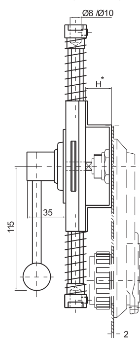
ZWPM10 (with hole \varnothing 10 )
