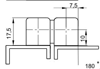
RIGHT VERSION
