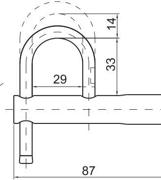
PADLOCK SN 4.KDSN.001
