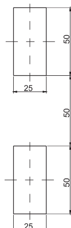
Mounting hole
