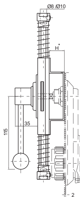
ZWPM10 (with hole \phi 10 ) \phi 8 / \phi 10
