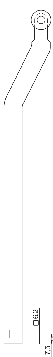
FLAT ROD WITH ROLLERSI A25K - L (with square hole)
