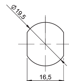
Mounting hole
