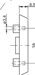
RW110.M ... (Used with Cogwheel mechanism)
