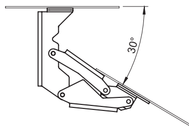
Open position
