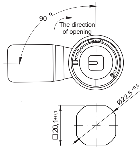
Cut out
