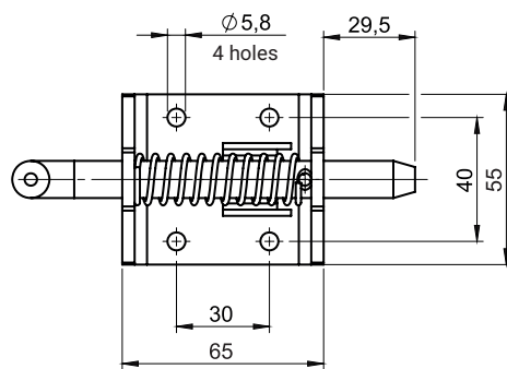
Locked Position
