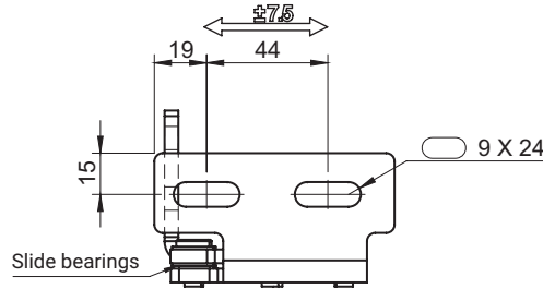
Closed position
