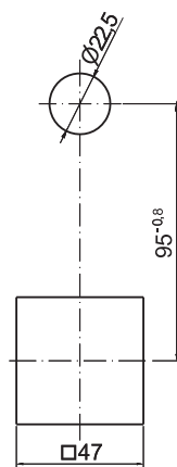
Mounting hole
