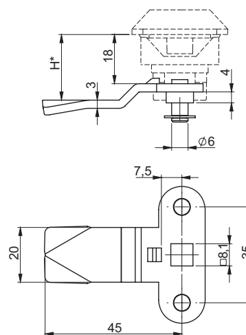
3-point CAM. (with limiter)
