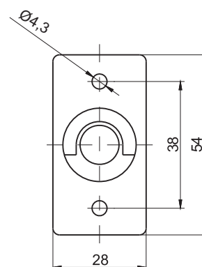
CAP 1C.902.001
