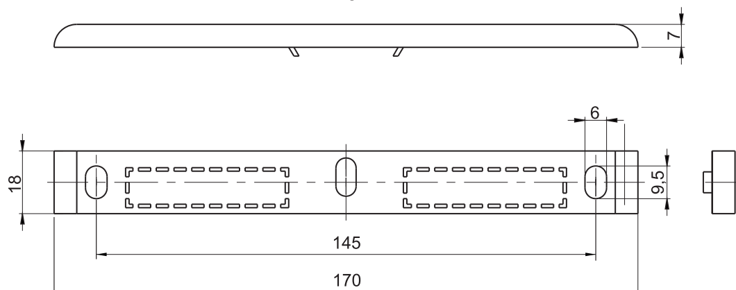
Masking element
