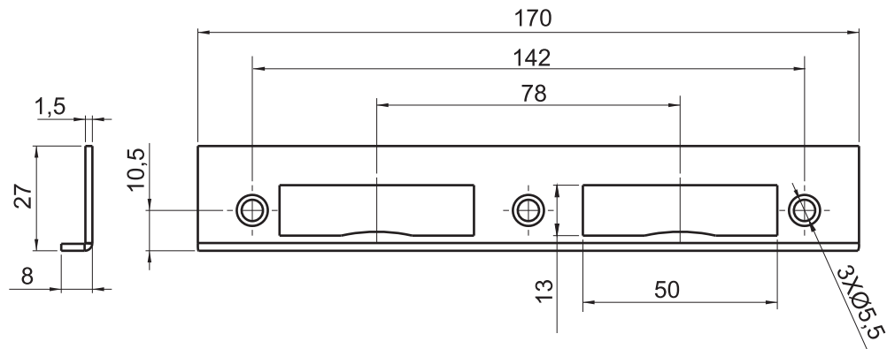
Latching element
