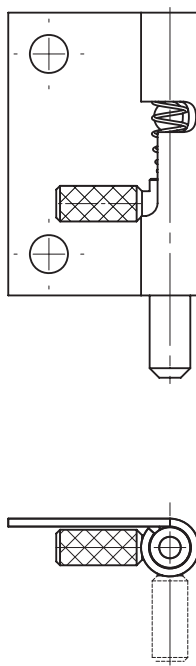
Right hinge 3.ST79.001
