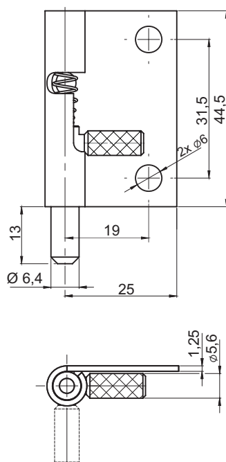
Left hinge 3.ST79.002
