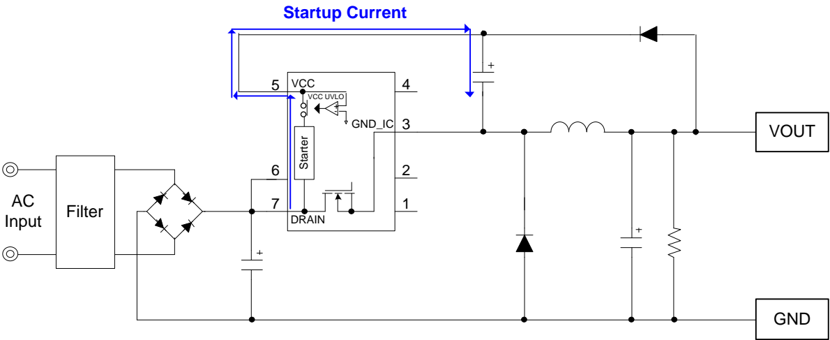
Figure 5. Startup Circuit
