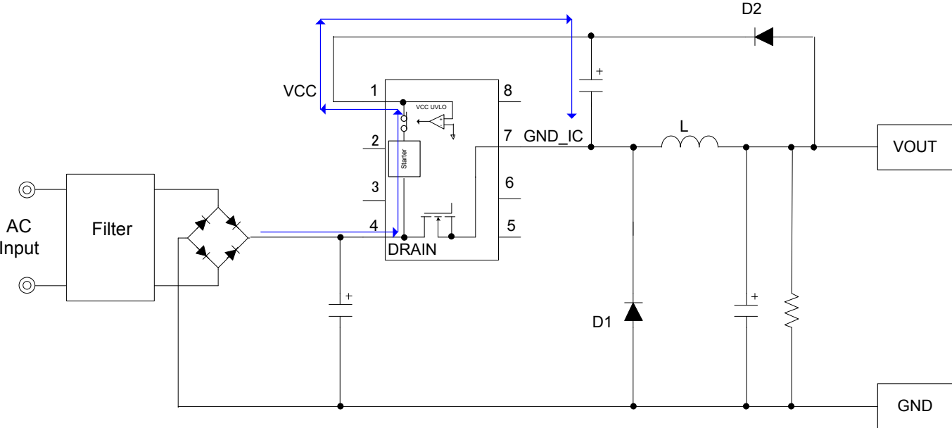
Figure 5. Start Circuit
