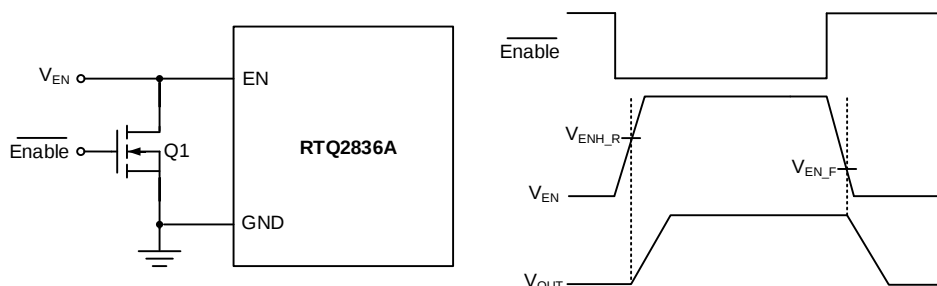
Figure 9. Logic Control for the EN Pin
