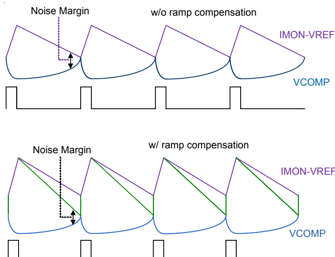
Figure 16. Ramp Compensation
