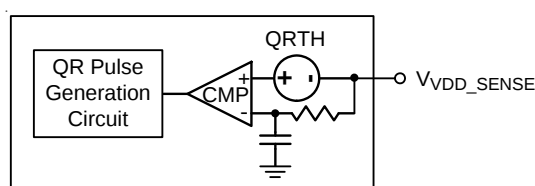
Figure 14. VDD Controller : Quick Response Triggering Circuit
